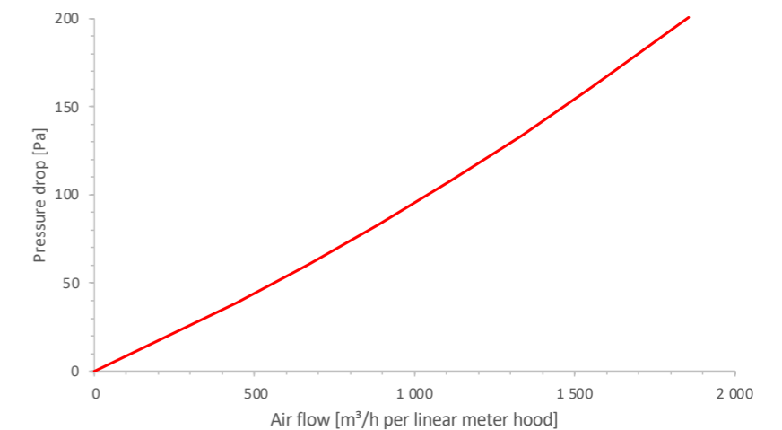
Pressure drop curve - Performair +
